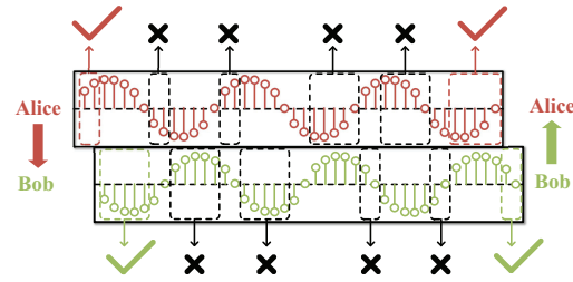
Fig. 4: When only few samples are available for dependent decoding, mZig is vulnerable to noise.
